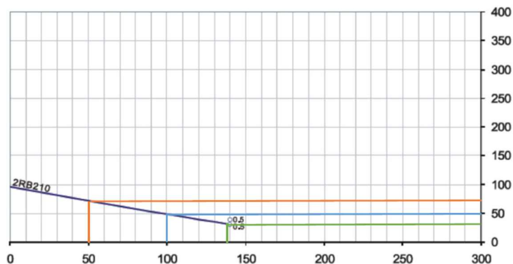
Compressor Selection Diagram 60Hz
