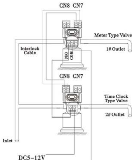
Figure 3-13 Series system
