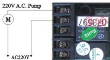
Figure 3-7Wiring of Booster Pump on Inlet
