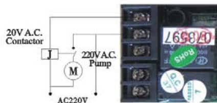
Figure 3-8 Wiring of Booster Pump on Inlet
