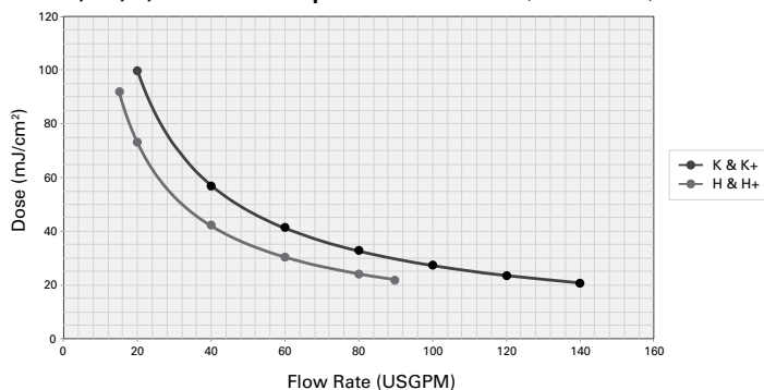
H, H+, K, & K+ Dose Response Curve at EOL (@ 95% UVT)
