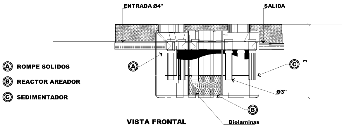
VISTA FRONTAL
